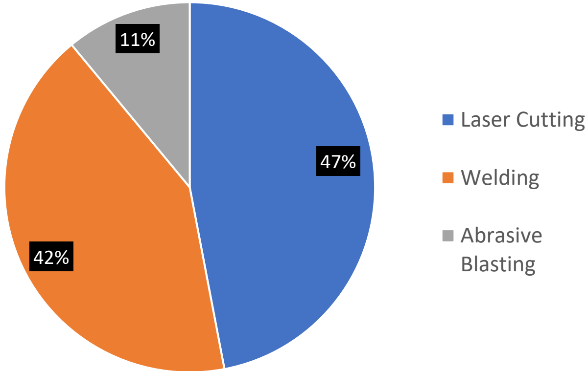
Source Contribution – Nickel Emissions (100% of Acute HHI)
